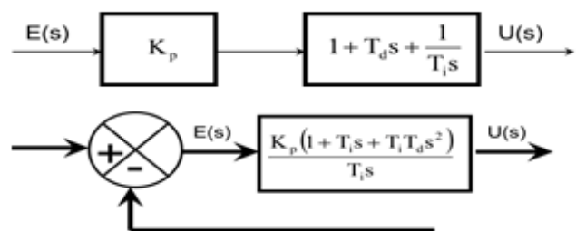
Fig.2 Block diagram of PID controller parameters
