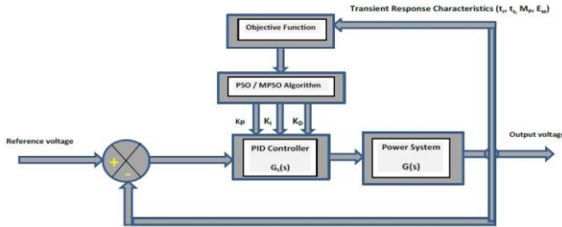
Fig 4. Block diagram of proposed PSO/MPSO-PID controller
