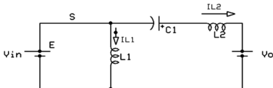
Fig. 2 Principle of Operation of Luo Converter
