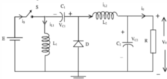
Fig. 1.Circuit diagram of Luo converter.
