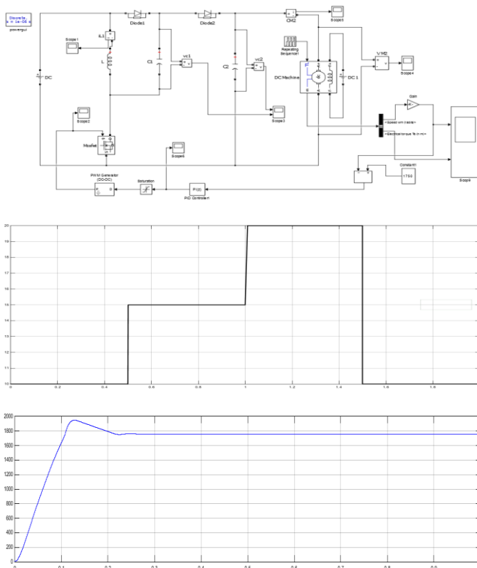
Fig. 5. Simulation of the Closed Loop Luo Converter
