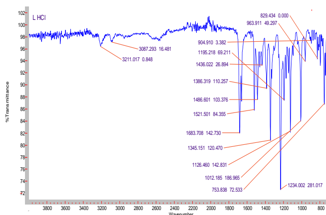
Fig. 2 FT-IR Spectrum of Lercanidipine HCl
