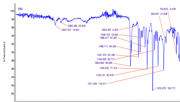
Fig. 4 FT-IR Spectrum of Prepared LER Physical Mixture (P2)
