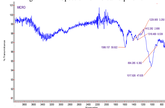
Fig. 3 FT-IR Spectrum of Prepared LER Microcrystals (F2)
